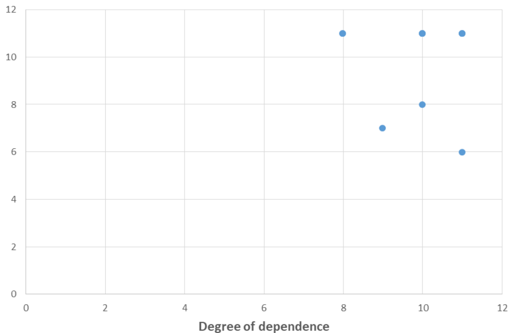
Figure 3. MICMAC analysis
